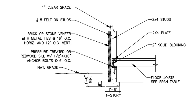
VENEERED WALL
