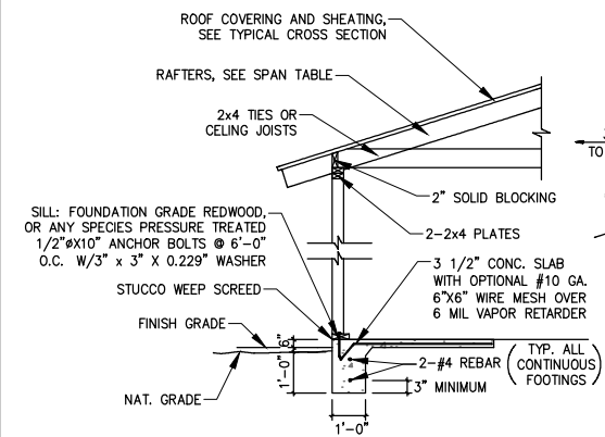
CONCRETE FLOOR
