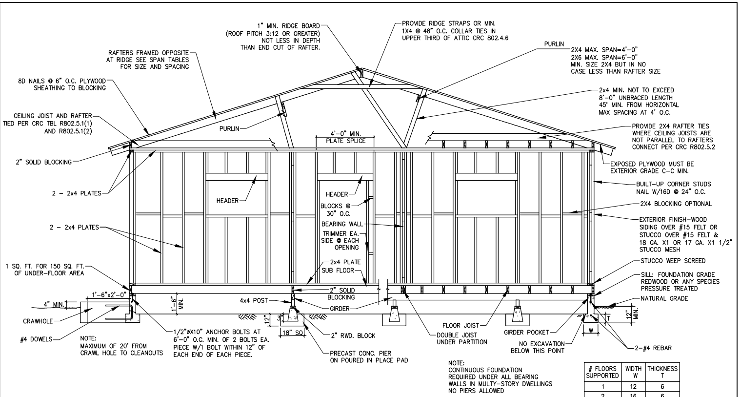
TYPICAL CROSS SECTION AT ENDWALL
