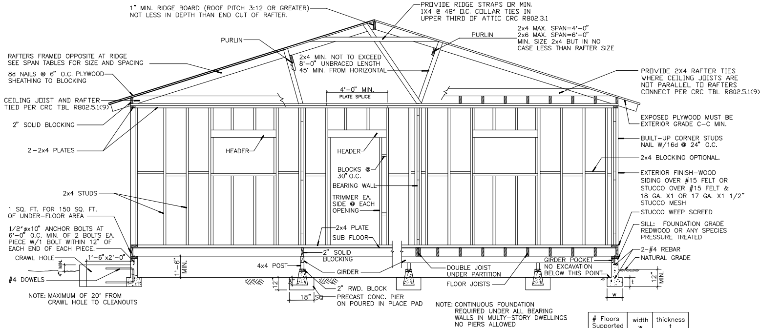
TYPICAL CROSS SECTION AT ENDWALL
